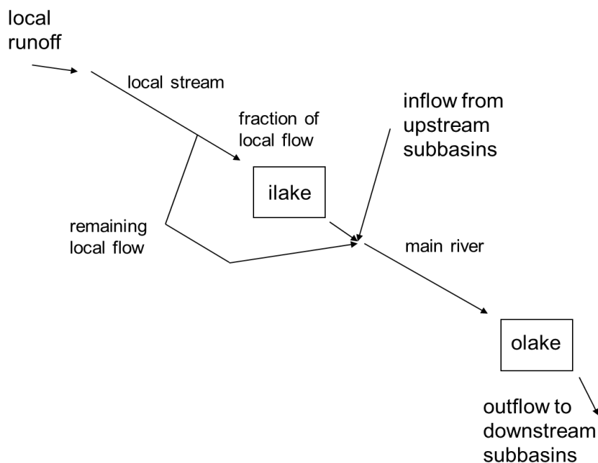
Figure 4. Water flow and calculation order from soil local runoff via local streams and lakes to the main river and outlet lake, and the coupling of upstream subbasin flow.
